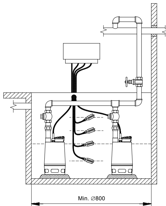
Fig. 30 Two-pump installation with four float switches
