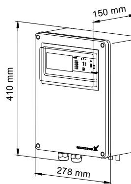
Fig. 53 Dimensional sketch, control cabinet
